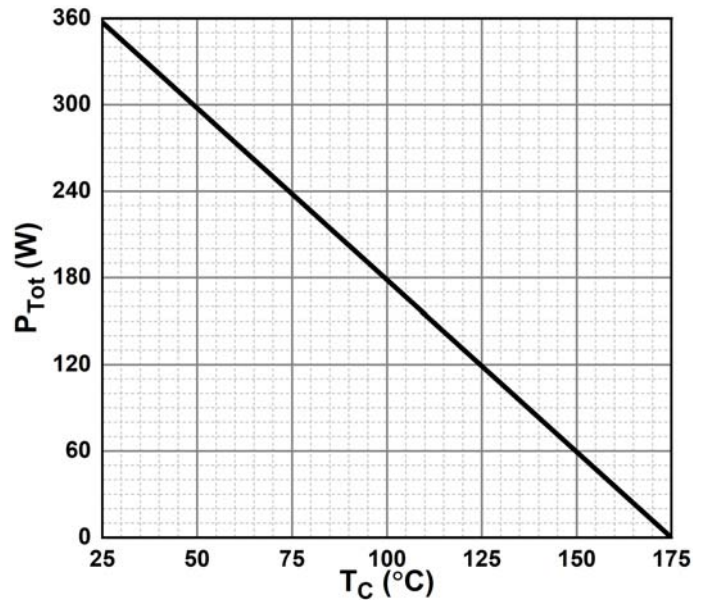
Figure 6. Power Derating
