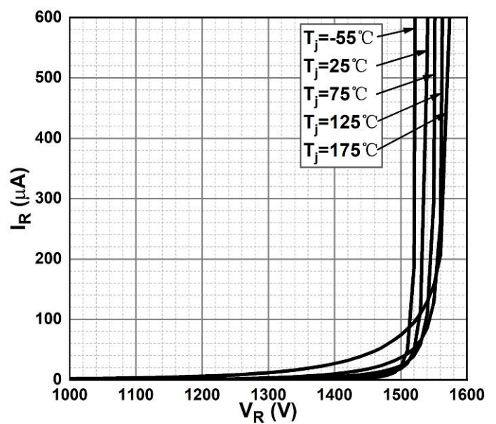
Figure 2. Reverse Characteristic
