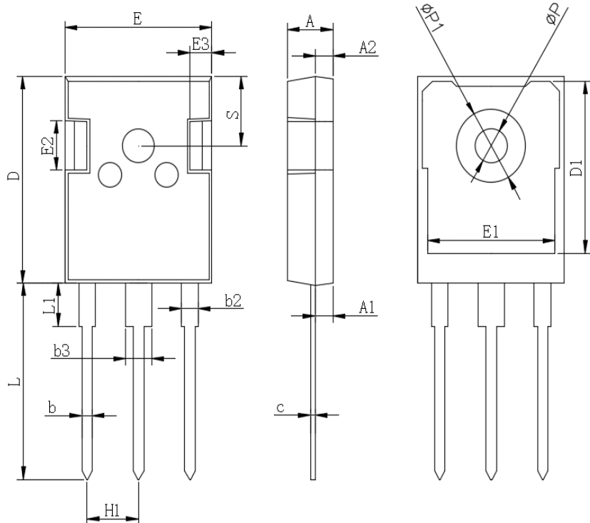
TO-247AB
